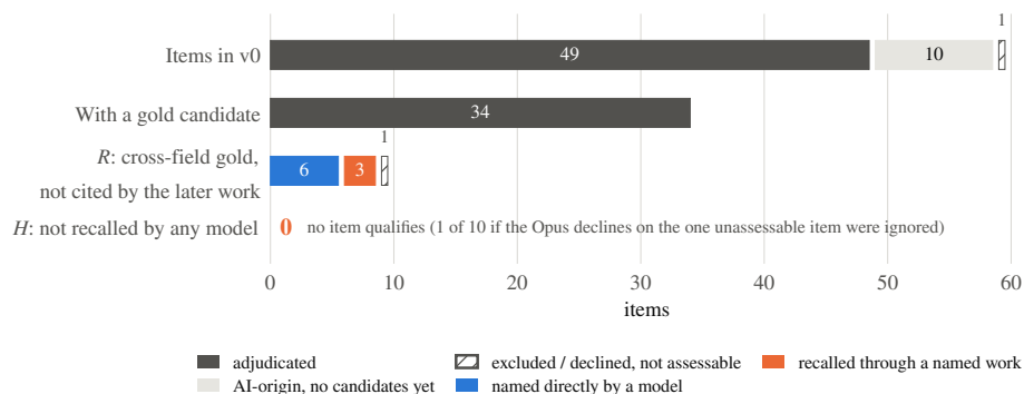
Fig. 2. From the items of v0 to H. Of 60 items, 49 carry adjudicated labels, 34 of them have a gold candidate, and 10 are in R. Nine of those ten are recalled by a model, six by naming a gold work directly and three through a work they named that the author judged cross-field gold; the tenth is not assessable because Opus 5.5 declined every sample. H is empty.
