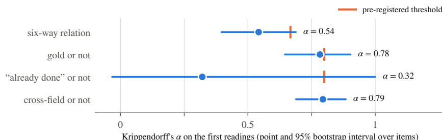
Fig. 1. Agreement of the quiz on the 136 pairs of b01 and b02. Points are Krippendorff’s alpha on the first readings and bars the 95% percentile bootstrap intervals over items (2,000 resamples); orange ticks are the thresholds of protocol decision 18 (none is set for cross-field status).
