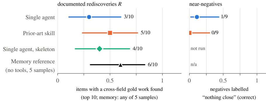
Fig. 3. Retrieval on R and labelling of the near-negatives. Left: items with a cross-field gold work found in the top 10 (memory reference: in any of five samples), with Wilson 95% intervals; gold includes the named works the author adjudicated. Right: near-negatives labelled nothing close , the correct label, for the two agents that were run on them.
